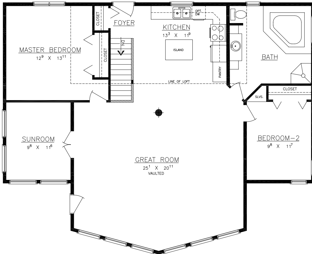
FLOOR PLAN
